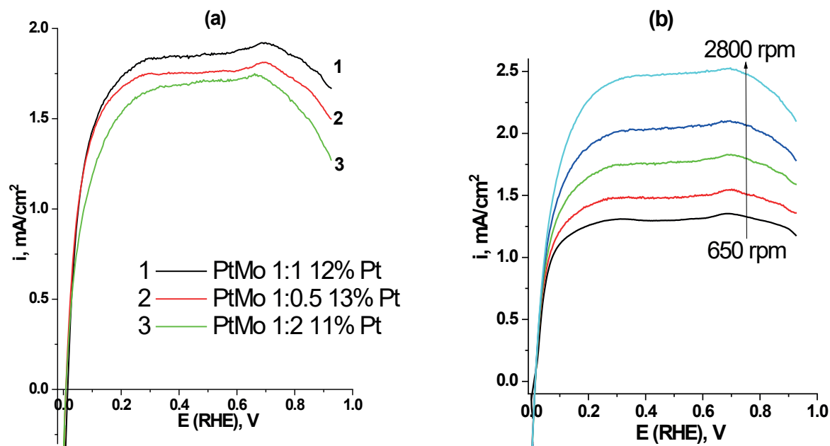
Fig. 15. a) Polarization curves of hydrogen oxidation on PtMo/CNTNaOH catalysts with different metal ratios in 0.1 M KOH. 0.005 V/s; 1500 rpm; m_{cat.} = 0.15 \text{ mg/cm}^2 . b) Polarization curves of hydrogen oxidation on PtMo/CNTNaOH catalyst with 12% platinum content at different electrode rotation speeds in 0.1 M KOH. 0.005 V/s; m_{cat.} = 0.15 \text{ mg/cm}^2
